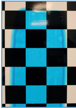
Fig. 4A Pigmented Polyurethane-based clear coating, without surface levelling additive Coating trasparente pigmentato a base PU, senza additivo livellante
